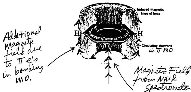
Figure 417. From "Spectrometric Identification of Organic Compounds," by Silverstein, Bassler, & Morrill, 5th Ed., Wiley, 1991
