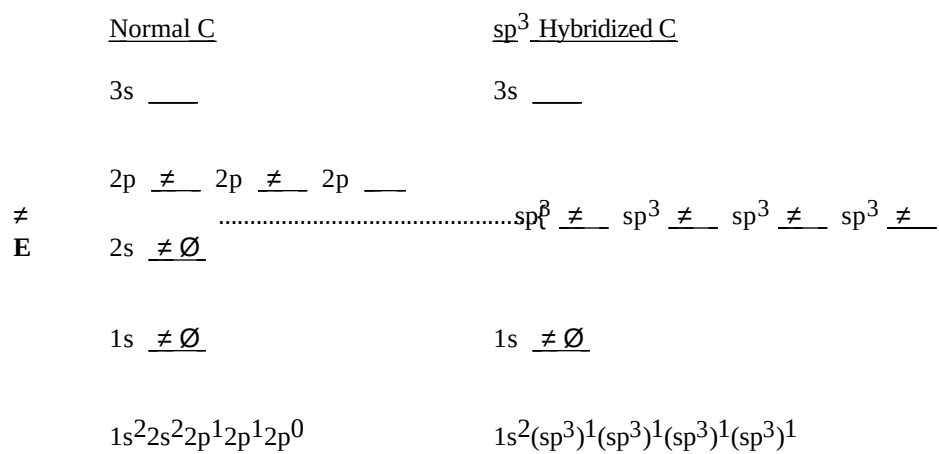
Figure [graphic 1.35]. Electron Energy Diagrams for Ground State and sp^3 Hybridized C.
