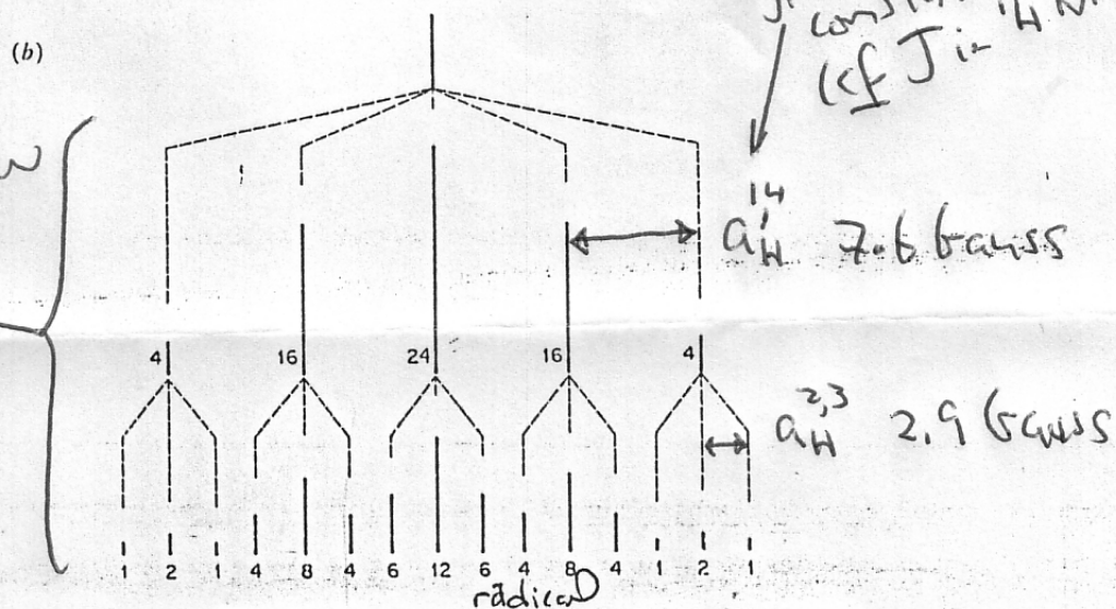
Fig. 4-13 (a) ESR spectrum of the butadiene anion in liquid \text{NH}_3 . [Spectrum kindly supplied by Professor R. J. Myers. See D. H. Levy and R. J. Myers, J. Chem. Phys. , 41 :1062 (1964).] (b) Reconstruction of the ESR spectrum of butadiene anion.
